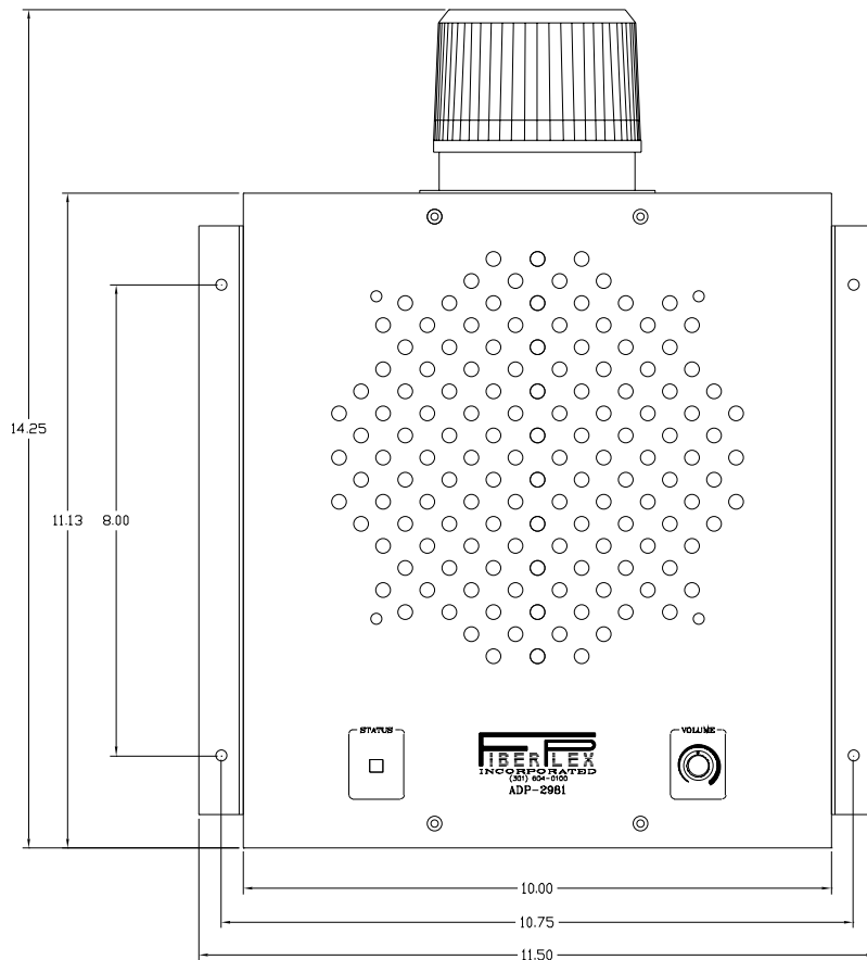
ADP-2981 Front View
